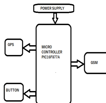
Figure 1: Block diagram for the components of tracking system
