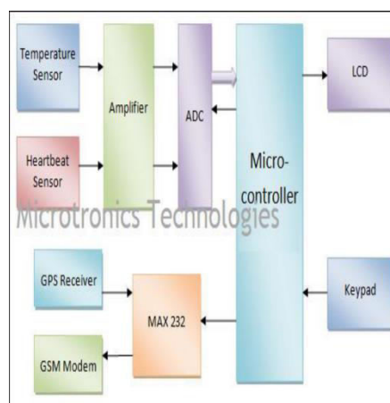
Fig shows the block diagram of soldier unit which includes following blocks.
