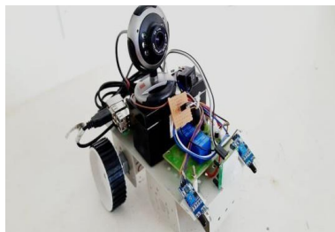
Fig9 Surveillance Robot
