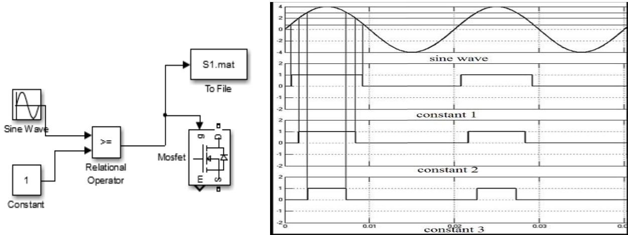
Fig.3 Proposed method for pulse generation
