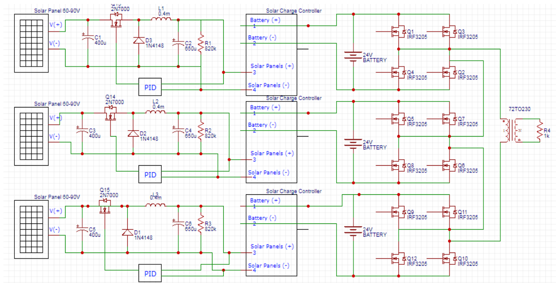
Fig.6 Complete circuit of the proposed system
