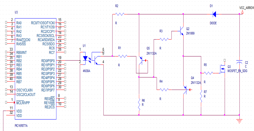
Fig.4 Push pull gate driver unit
