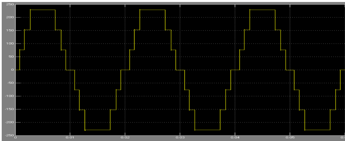
Fig.8 Simulation result of 7 level inverter
