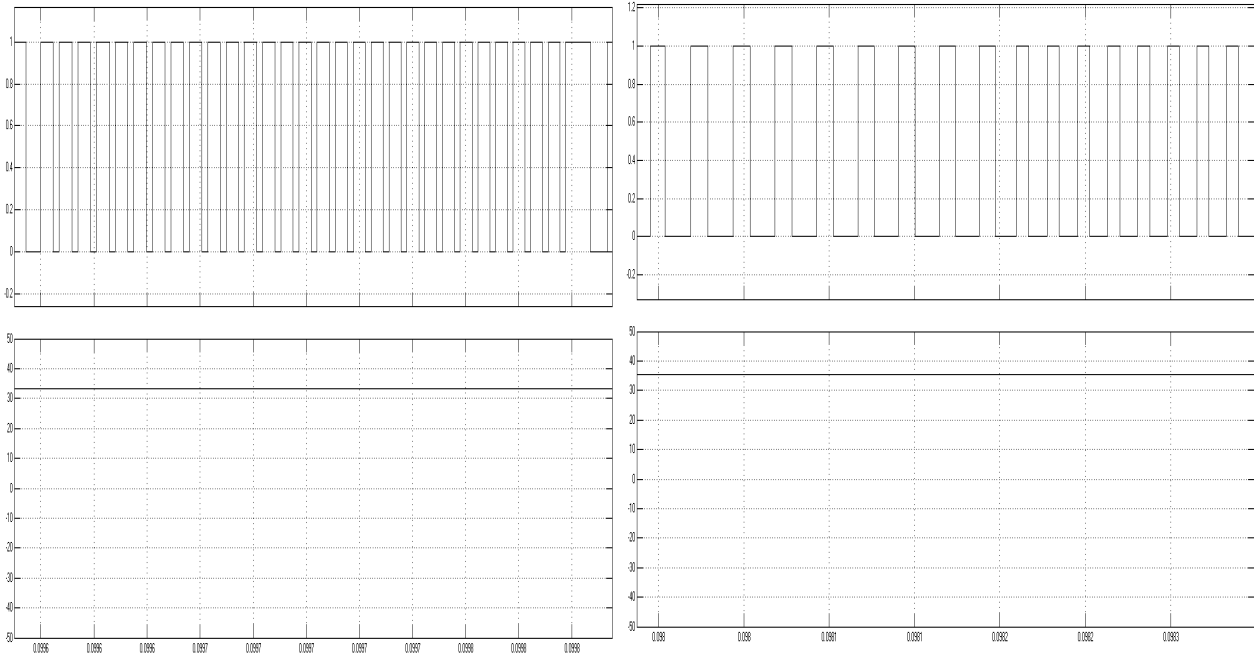
Fig 10 Simulated result of closed loop buck converter
