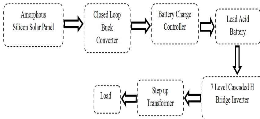
Fig.1 Block diagram of the complete system
