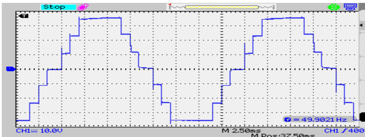
Fig 9 Hardware tested result of output waveform
