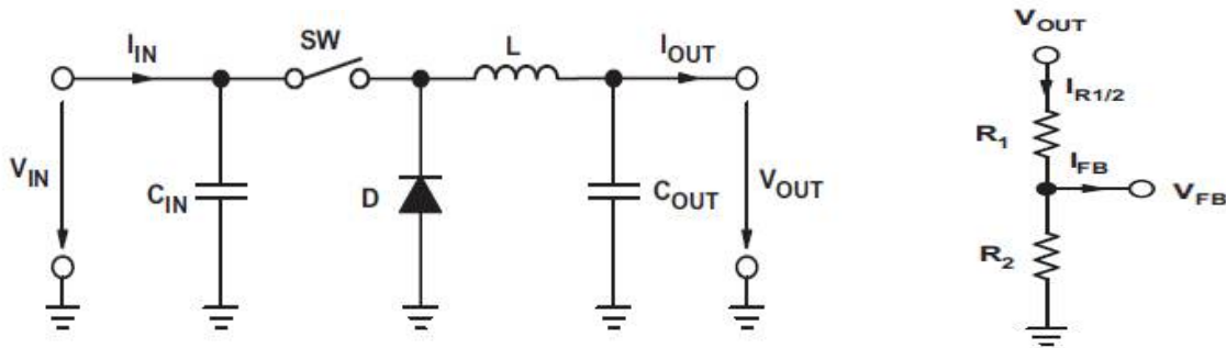
Fig.5 Buck converter with feedback circuit
