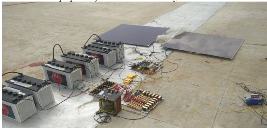
Fig.7 Hardware implementation
