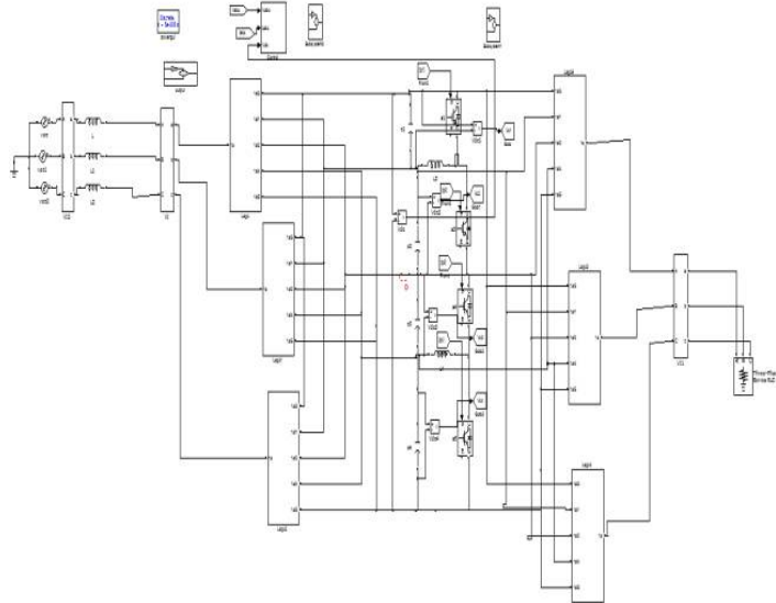
Fig.8.Matlab/Simulation model of Proposed 5L bidirectional ac/dc/ac drive based on multiple-pole multilevel diode-clamped converter (5L-M 2DCC) approach.
