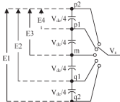
Fig. 4. Circuit diagram of per phase leg single-pole classical 5L-MDCC topology with switching position.
