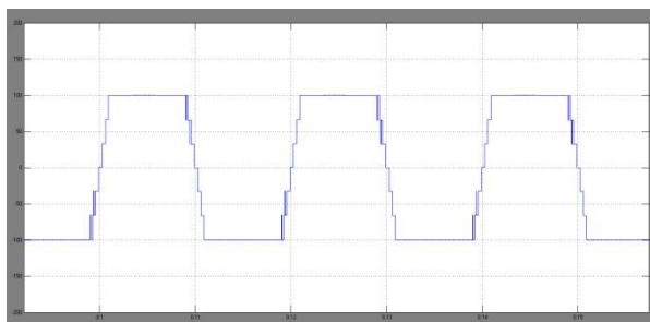
Fig.14.shows the output voltage of the proposed seven level inverter.
