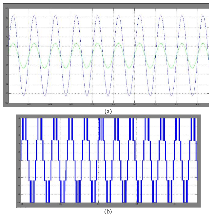
Fig. 9. Unity power factor operation with rectifying mode. (a) Voltage and current at the grid side. (b) Pole voltage at the rectifier side.
