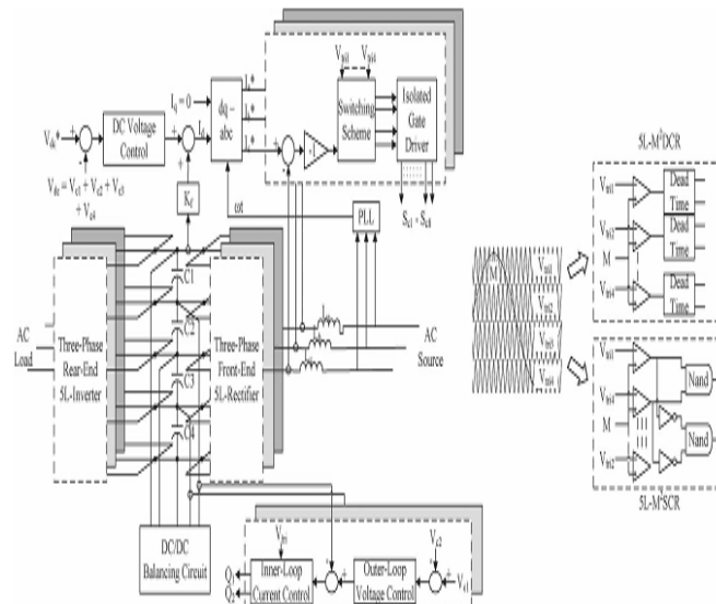
Fig. 7. Proposed front-end rectifier controller for the 5L ac/dc/ac converter.
