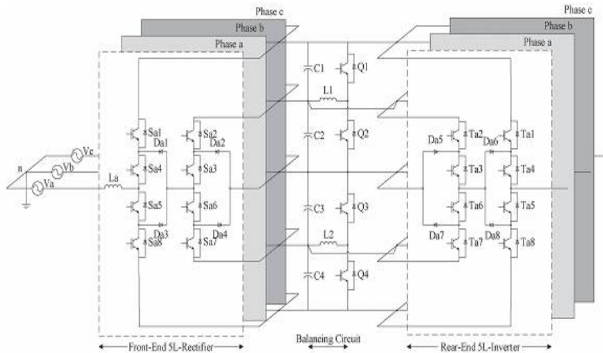
Fig. 1. Proposed 5L bidirectional ac/dc/ac drive based on multiple-pole multilevel diode-clamped converter (5L-M2DCC) approach.
