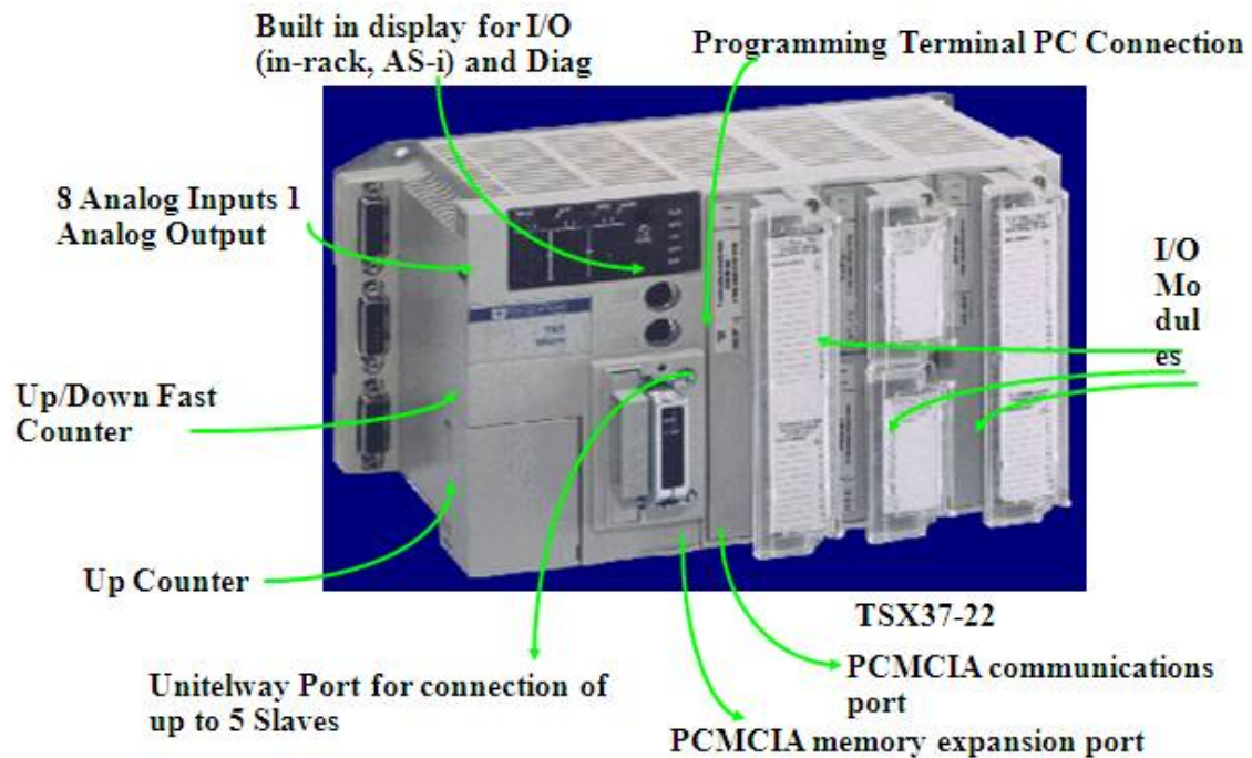
Fig 3.2 Configuration of Modicon PLC
