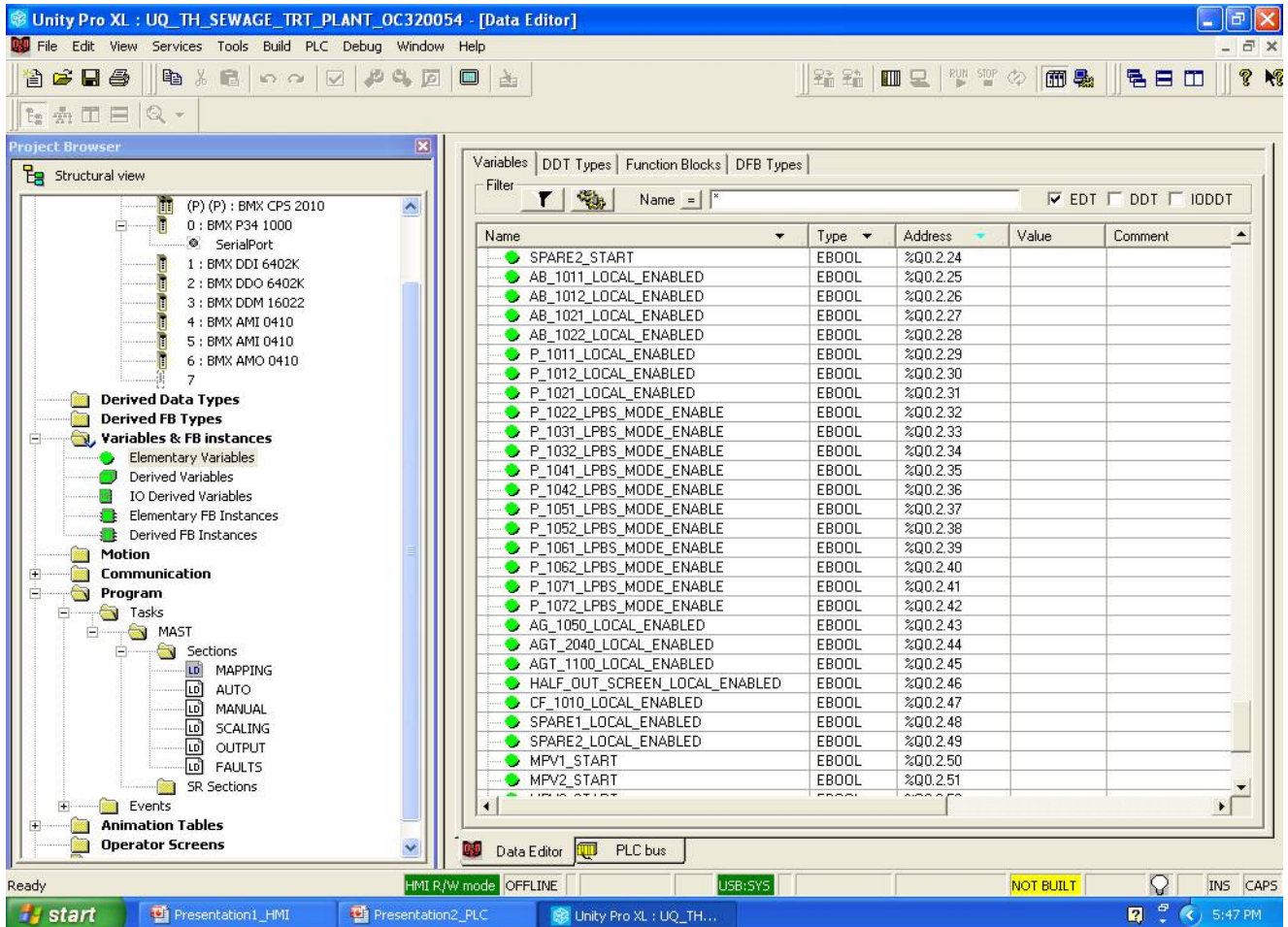
Figure 5.1 (b): - Digital Output Mapping Using Structural Text Programming
