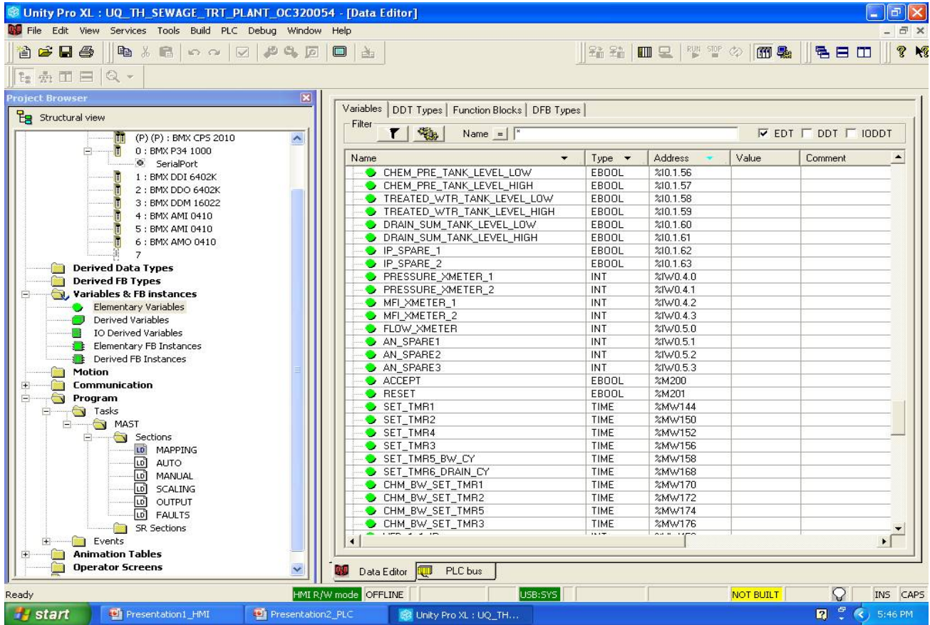
Figure 5.2: - Analog Input Output Mapping Using Structural Text Programming
