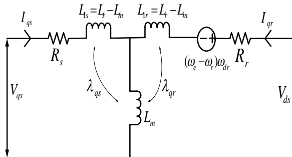
Fig.2: Dynamic equivalent circuit of SEIG (q-axis circuit)
