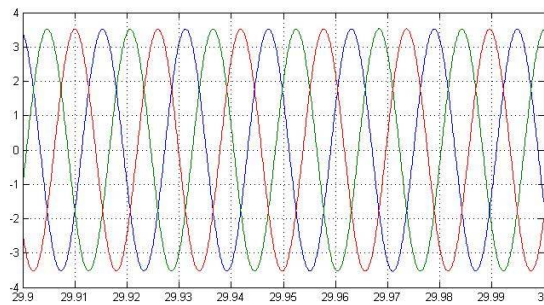
Fig.9: Steady-state response of SEIG load currents
