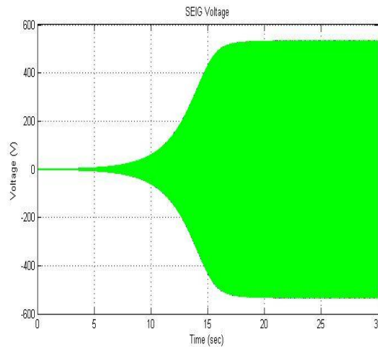
Fig.4: Transient response of SEIG voltages
