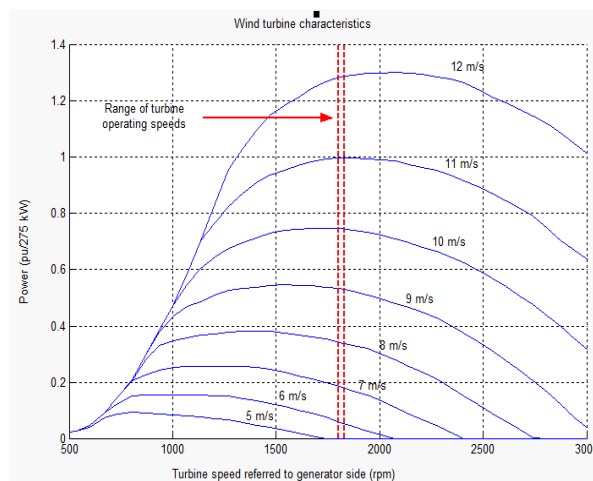
Fig.14: Simulink result of Wind Turbine Characteristics
