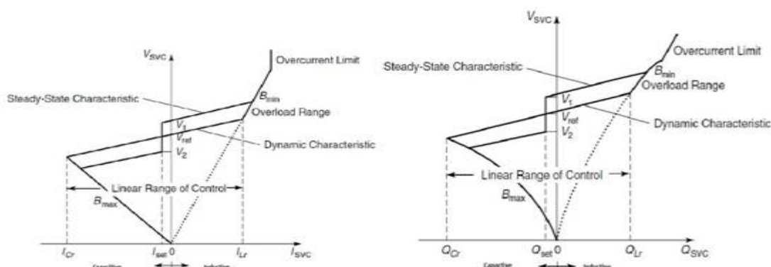
Figure 10(a) The voltage–current characteristic of the SVC and (b) the voltage– reactive-power characteristic of the SVC.
