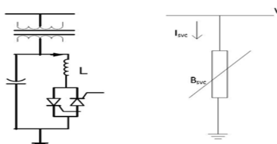
Fig. 9 Static var compensator and its equivalent circuit
