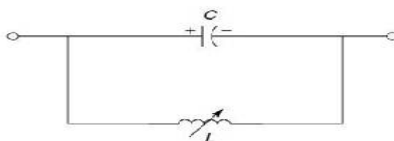
Fig 6 A variable Inductor connected in Shunt with an FC
