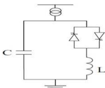
Figure 11 Basic SVC topology
