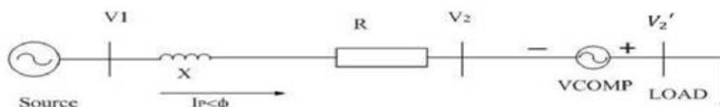
Figure 1 Representation of AC system with series compensation
