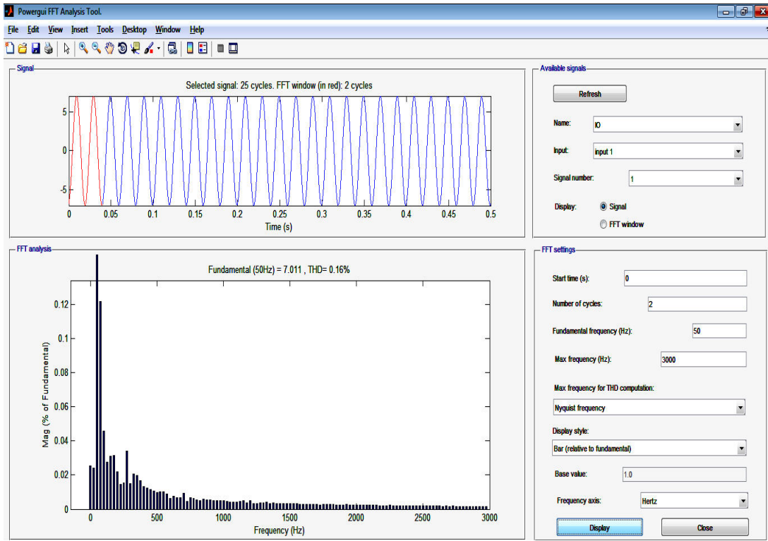
Figure 5: THD for bus 9 current waveform
