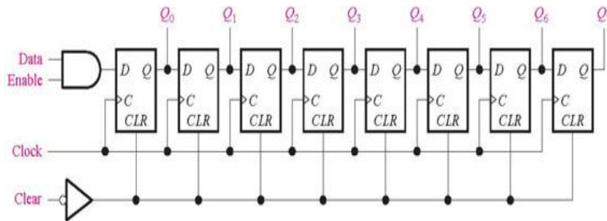
Fig. 3.3 8-bit shift register of Parallel input and serial output method
