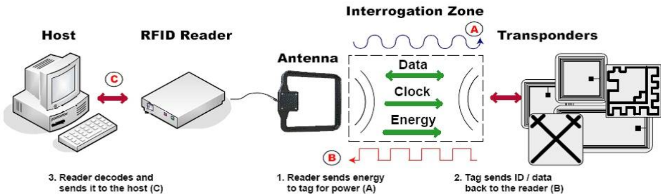
Figure3:RFID communication system.
