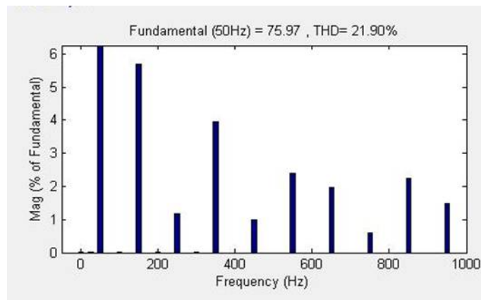
Fig 15 Reduced THD of grid voltage
