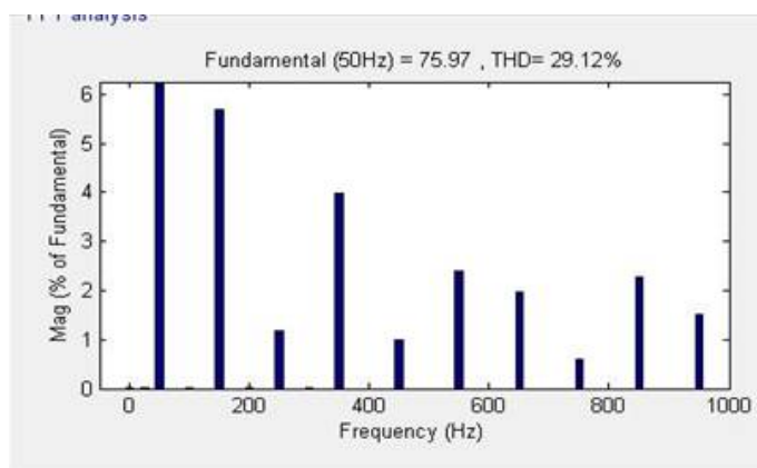
Fig 13 THD of grid voltage
