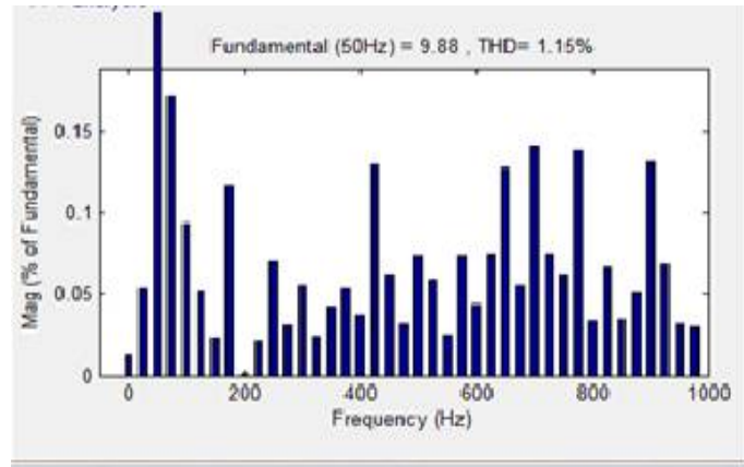
Fig 14 THD of grid current
