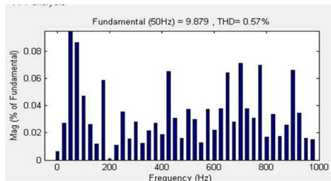
Fig 16 Reduced THD of grid current
