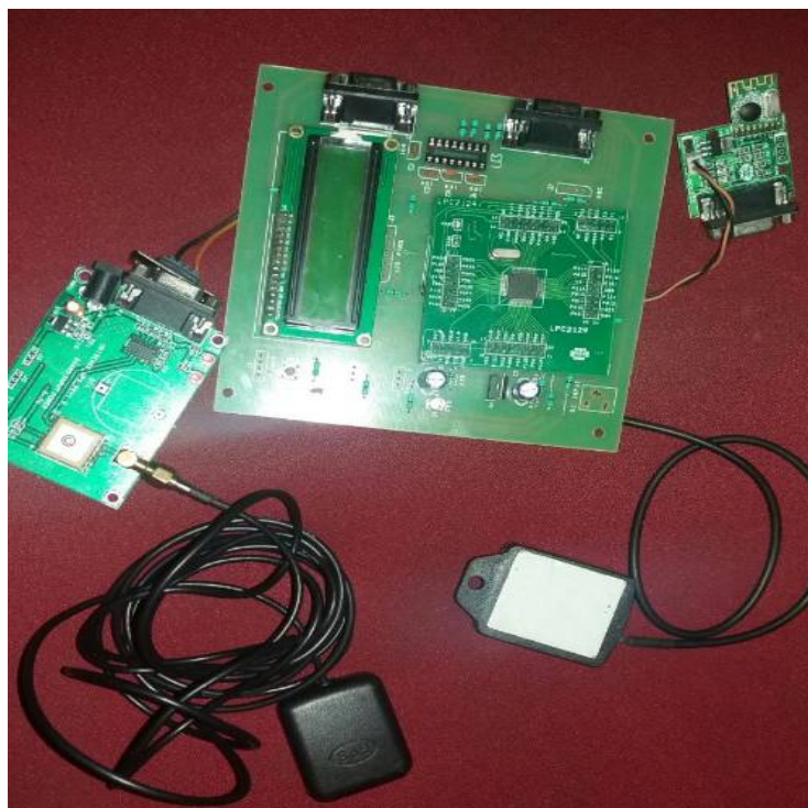
Fig1. Shows the snapshot of the (VOBU) Vehicle On Board Unit
