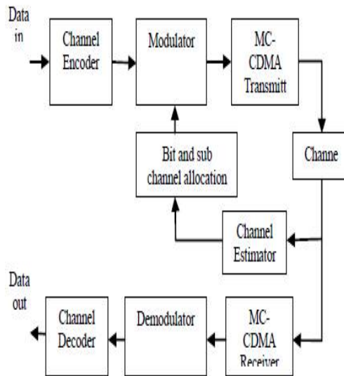
Figure1. MC-CDMA system
