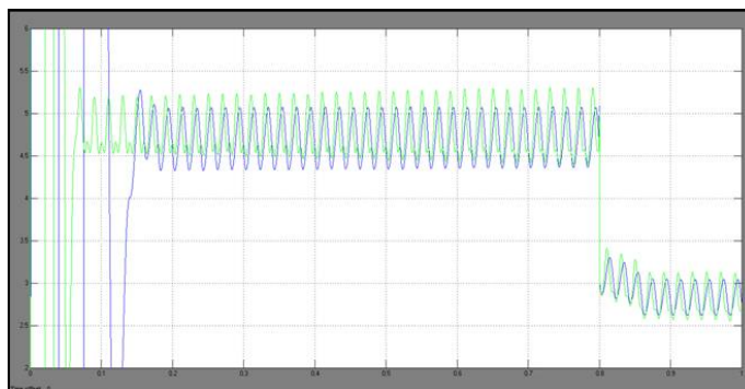
Fig 7: pv currents of phase a with distributed mppt(t=25).
