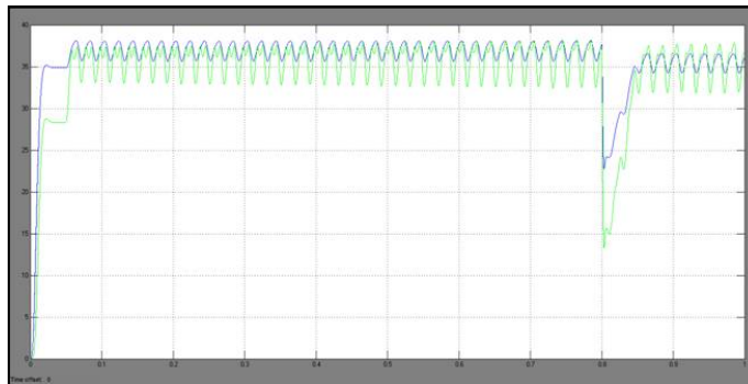
FIG 5:dc link voltage of modules 1 and 2.
