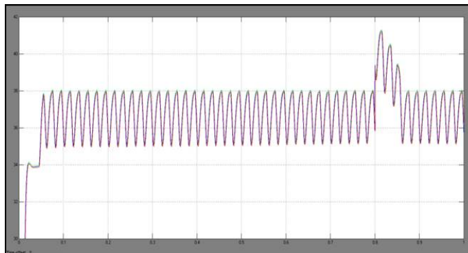
Fig. 6 Dc link voltage of module 3.
