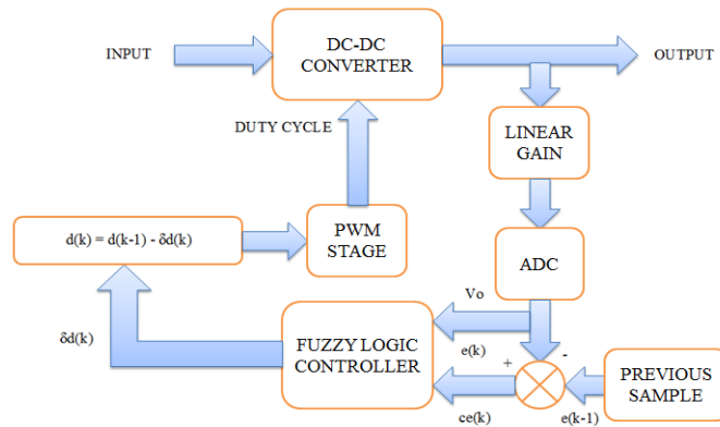
Fig. 2. Buck-Boost Converter Using Fuzzy Logic Controller
