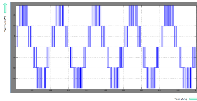
Fig. 6. Five – Level Inverter Output
