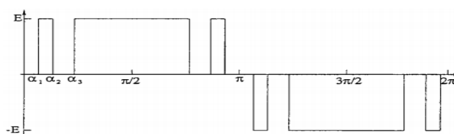
Fig.2 Three pulse PWM waveform.
