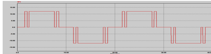
Fig.4 PSIM -PWM waveform window
