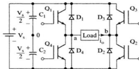
Fig.4 Full bridge inverter circuit
