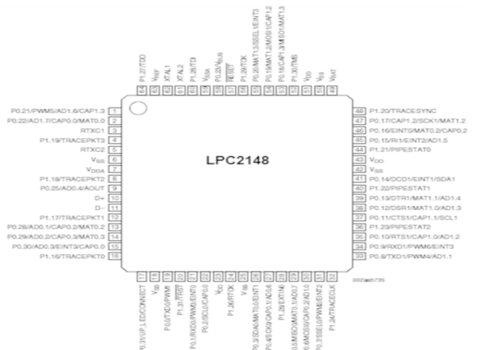
Fig. 4 LPC2148Microcontroller
