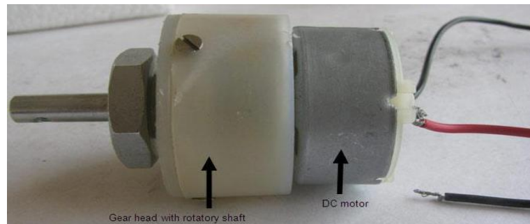
Fig. 7 DC Geared motor
