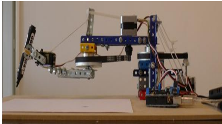
Fig. 9 Writing Robotic Arm by Speech Recognition
