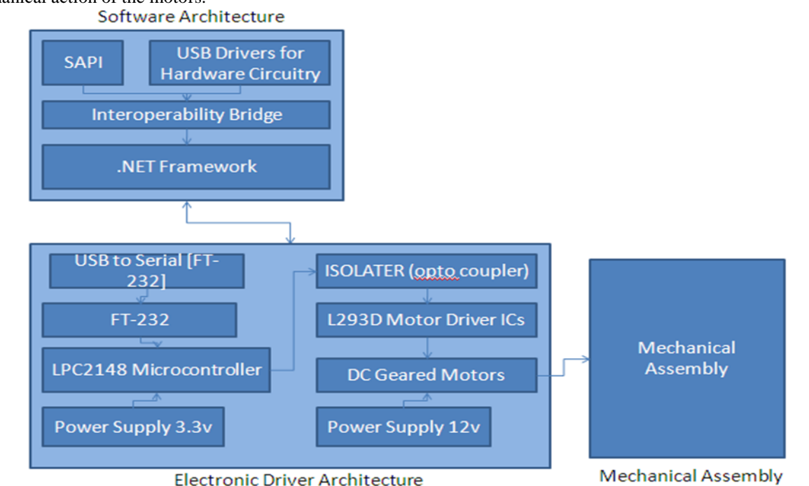
Fig. 3 Block diagram
