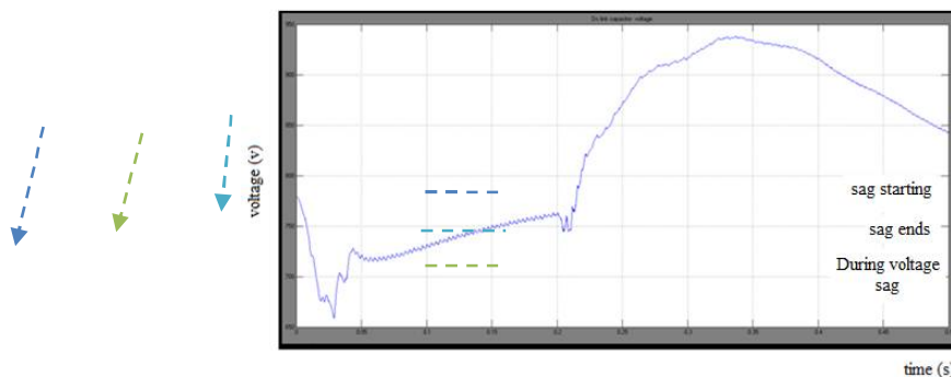
Fig. 6. Variation of the dc-link capacitor voltage before and during the 20% of voltage sag.
