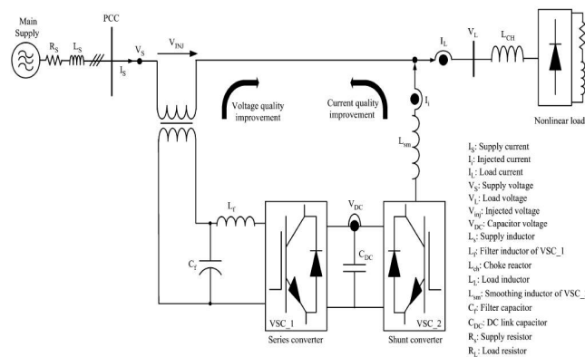
Fig. 1. Schematic diagram of UPQC.
