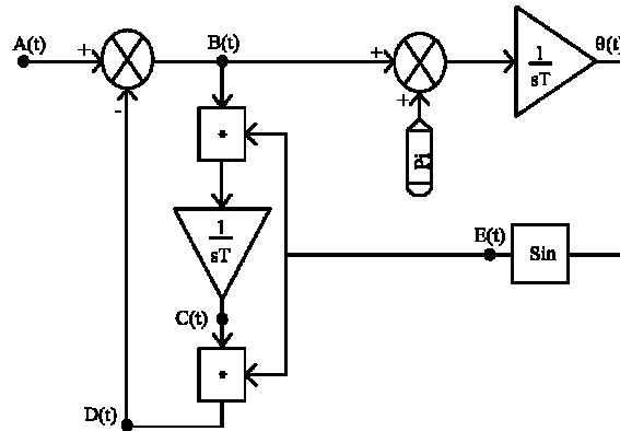
Fig. 3. Block diagram of the proposed algorithm.
