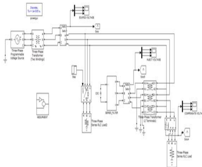
Fig. 5 Test System With Series Converter.
