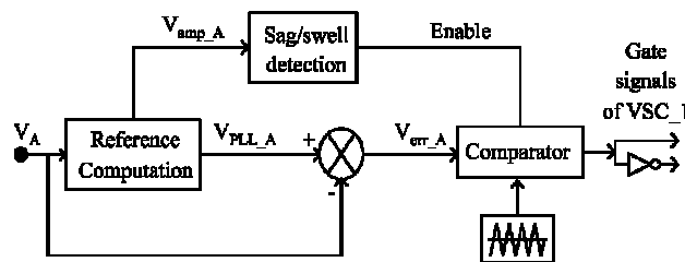
Fig. 2. Control block diagram of the series converter.
