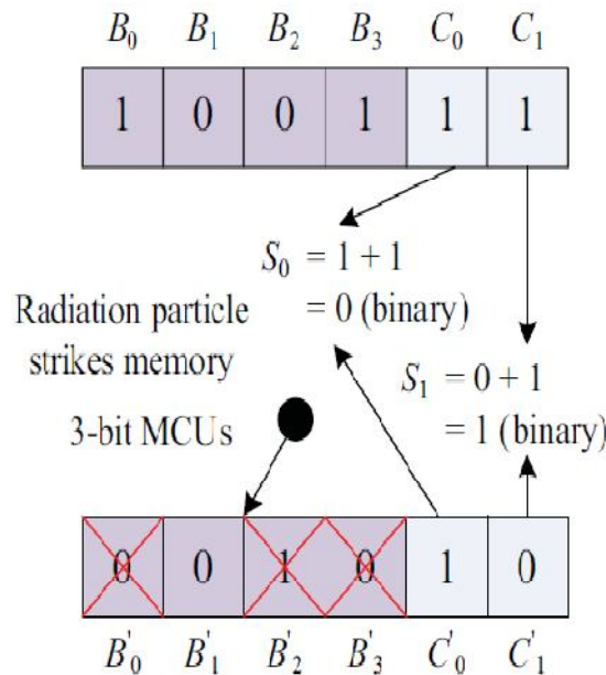
Fig 5 : limits of binary error detection in simple binary operations
