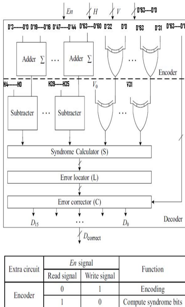
Fig 4: 64-bit DMC decoder structure using ERT
