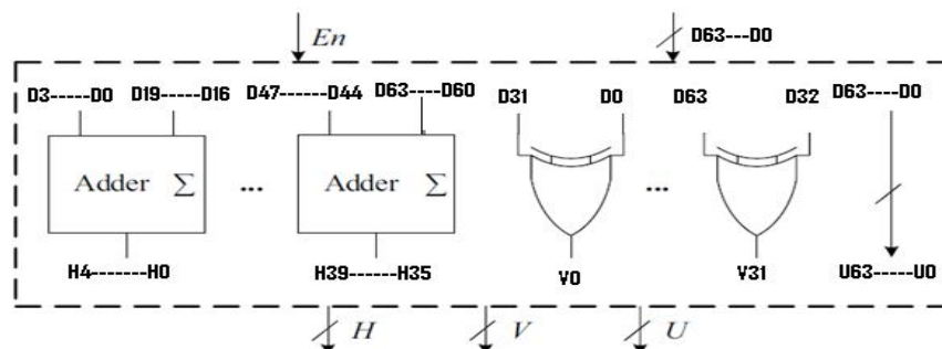
Fig 2: 64-bits DMC logical organization (k = 2 × 8 and m = 4). Here, each symbol is regarded as a decimal integer
