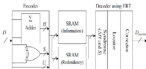
Fig 1: Proposed schematic of fault-tolerant memory protected with DMC.
