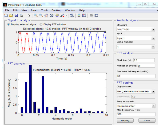
FFT analysis using PID controller
