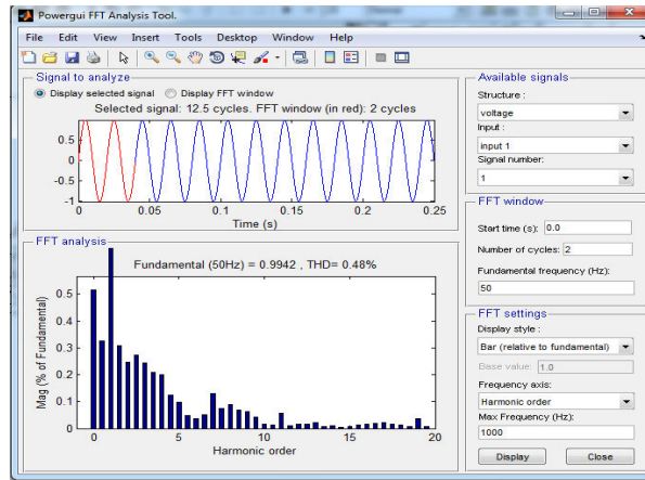
FFT analysis using Fuzzy Logic Controllers
