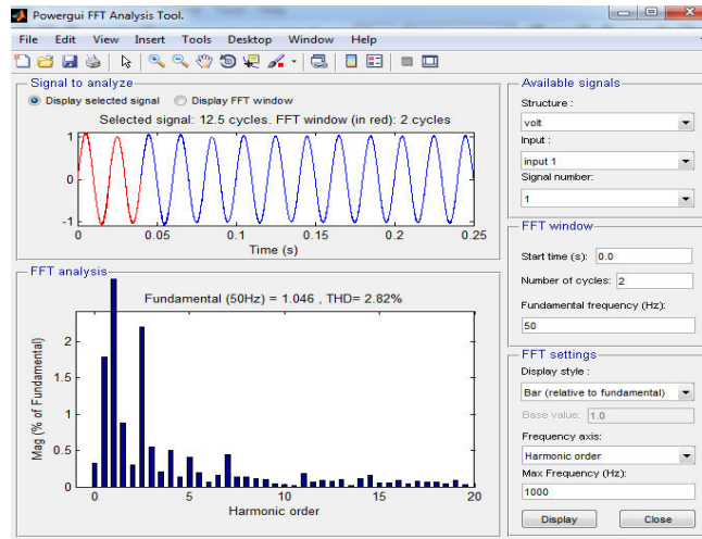
FFT analysis using PI controller
