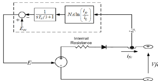
Figure:4. Equivalent circuit of fuel cell stack
