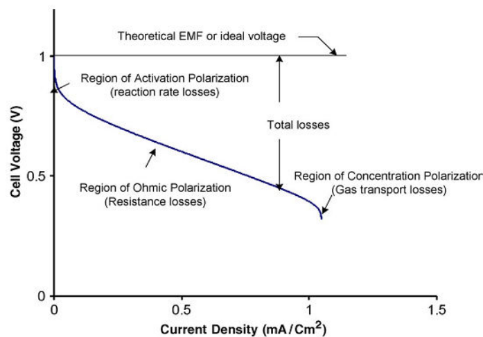
Figure: 3.Polarisation characteristics of fuel cell
