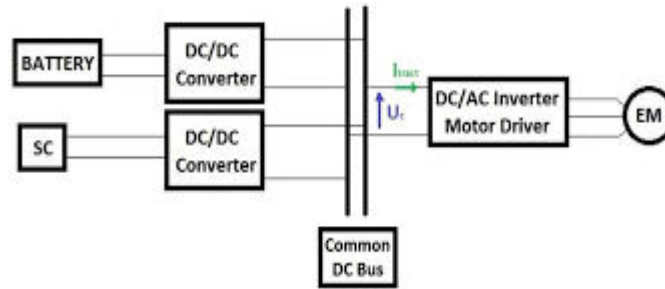
Figure 1: HESS of Electric Vehicle
