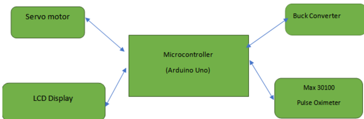
Figure 1: Block Diagram of the Project
