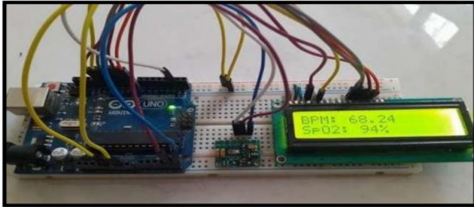
Figure 1 : Testing of max30100 and implementation on bread board is successfully worked.
