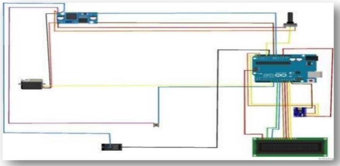
Figure 2: Circuit Diagram of the Setup
