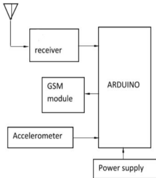
FIG. 1.4 Receiver Unit
