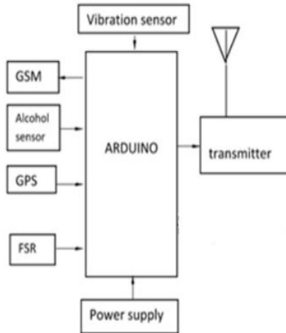
FIG. 1.3 Transmitter Unit
