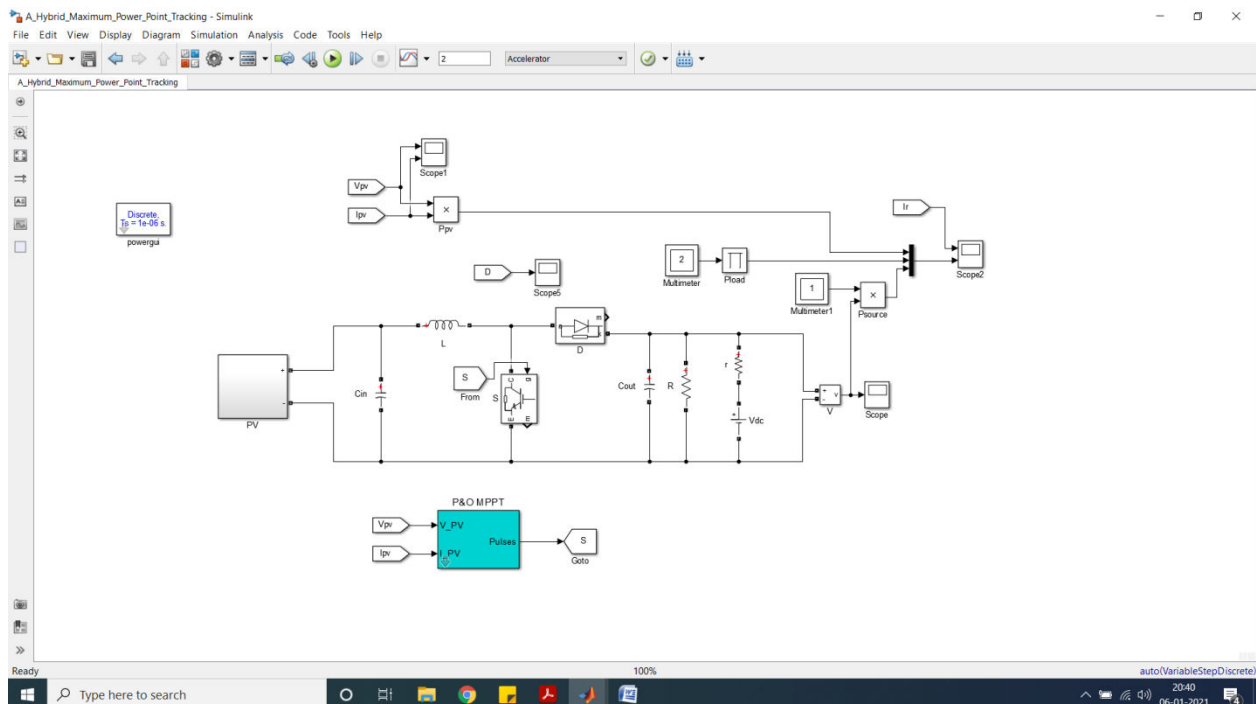
Fig. : 5 Proposed test system with four PVA module and P&O MPPT
