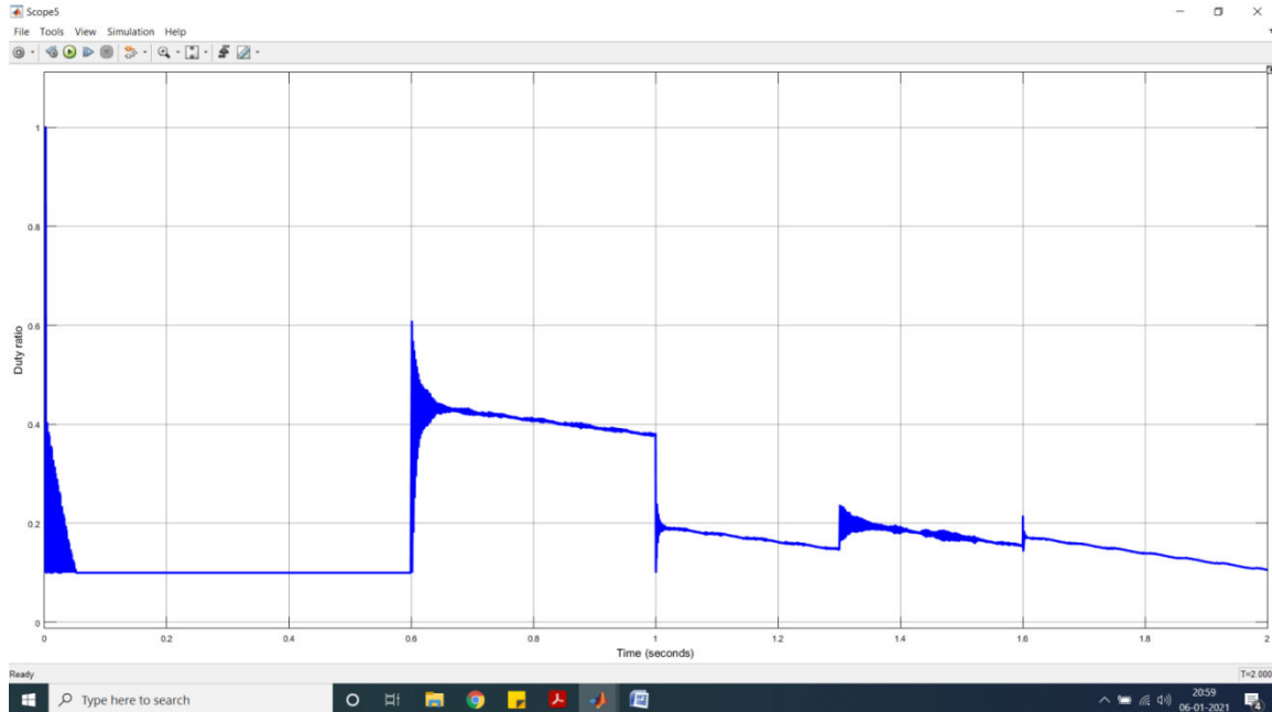
Fig.10 : Duty ratio of the boost switch
