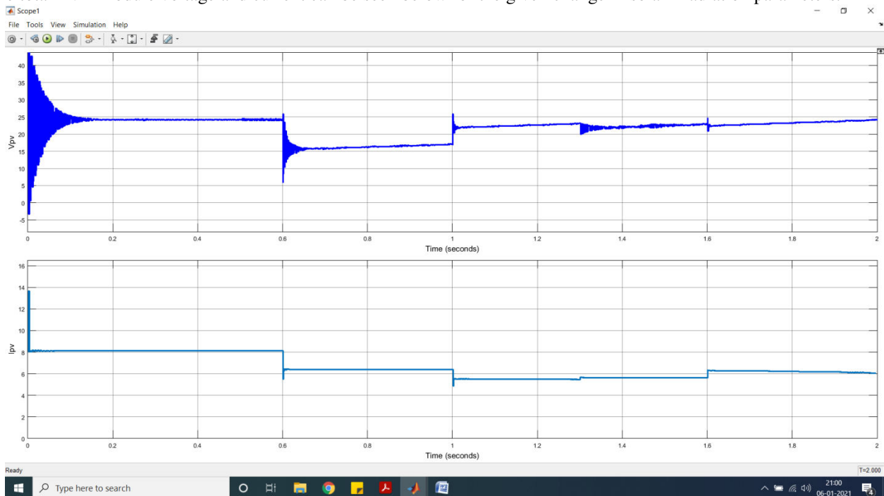
Fig11. : PVA module voltage and current output
