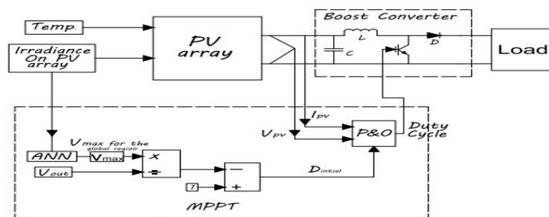
Fig 3: Proposed block diagram
