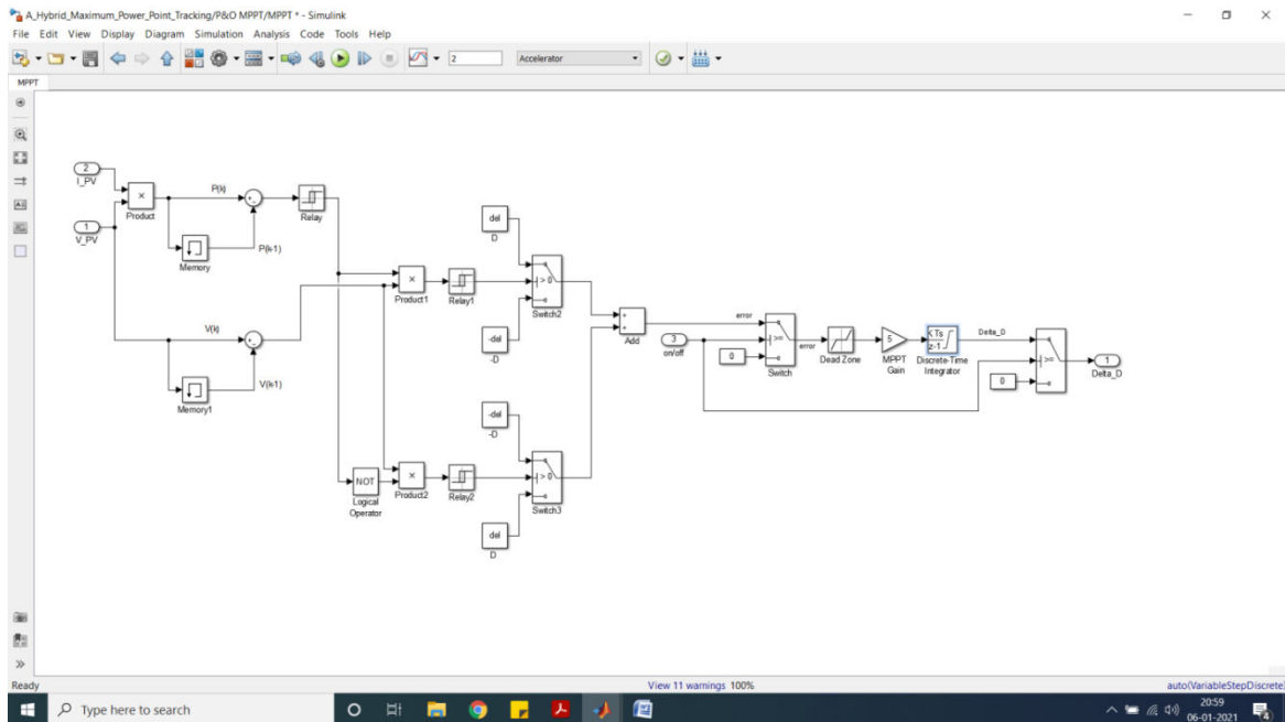
Fig. 7: P&O MPPT method modelling
