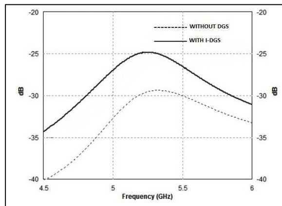
Fig. 5. Mutual Coupling S_{21} without and with I-shaped DGS.
