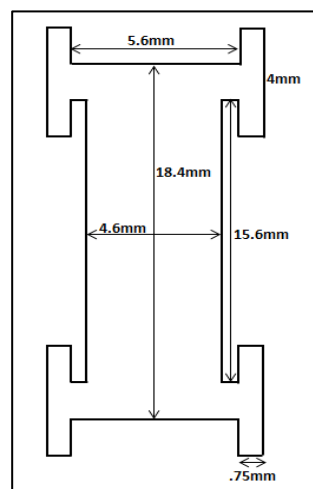
Fig. 3. Optimized dimension of I-shaped DGS for Fig-2 (b).
