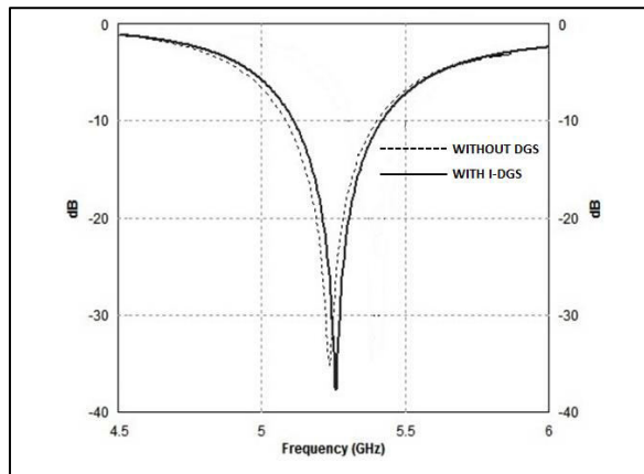
Fig. 4. Return Loss S_{22} , without and with I-shaped DGS.
