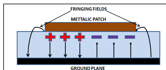
Fig-1. Schematic of Micro strip Antenna showing fringing fields.
