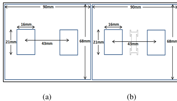
Fig. 2. (a) Dual patch antenna without I-shaped DGS. (b) Dual patch antenna with I-shaped DGS.
