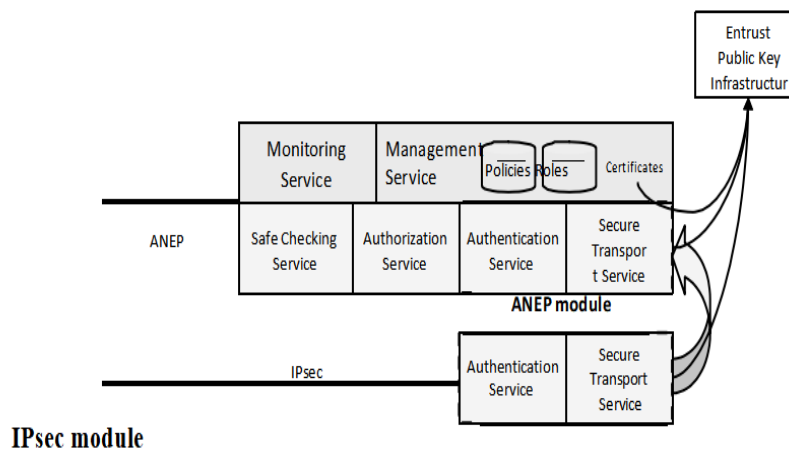
Figure 2 : The PNC architecture of security services
