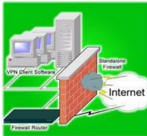
Figure 4 : Firewall
