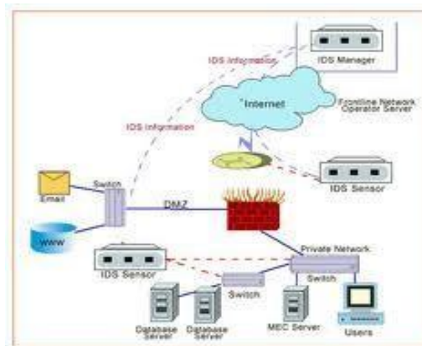
Figure6 : Intrusion Detection
