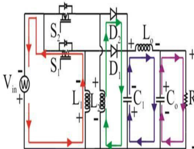
Fig3.4Fourth Mode
