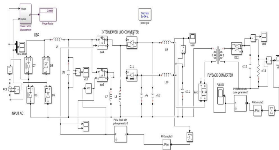
Fig 4.2 Simulation Diagram
