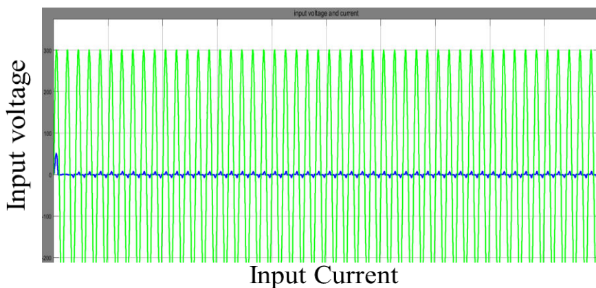
Fig 5.1 Input voltage And Current For Luo Converter
