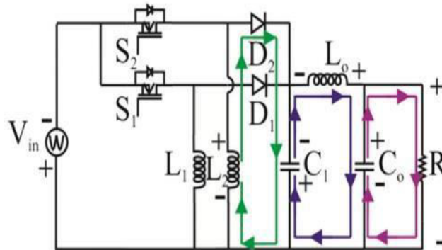
Fig3.3Third Mode
