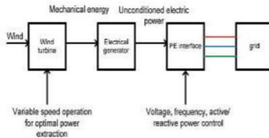
Figure 3: Variable speed wind energy conversion system
