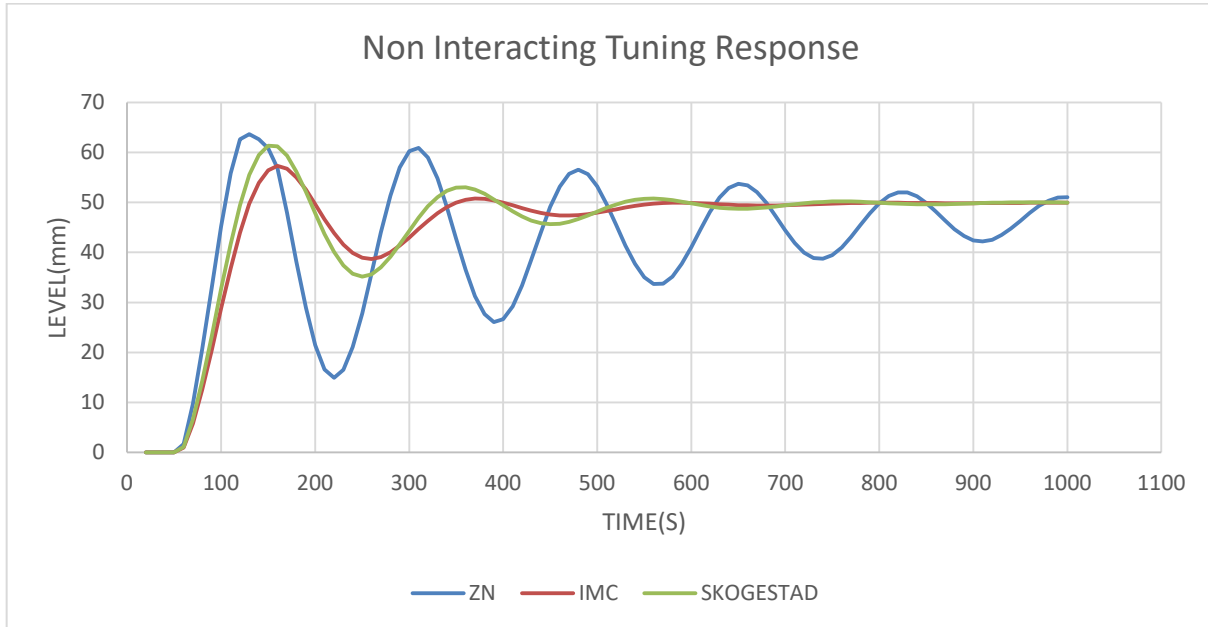
Figure 7 Closed loop tuned responses
