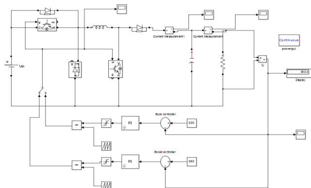
Fig.6. Boost/buck converter
