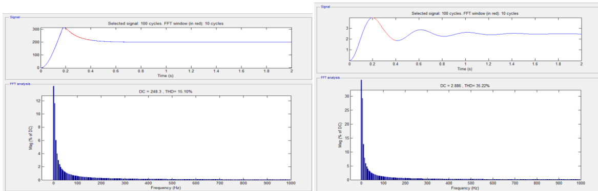
Fig.14. Fft analysis for buck boost converter with ivff
