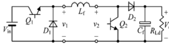
Fig. 1. Two-switch buck-boost (TSBB) converter.
