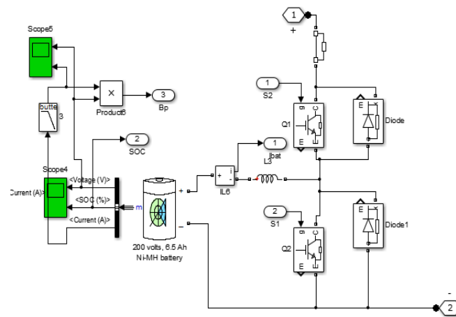
Figure 8: MATLAB Model for Battery and DC-DC Converter
