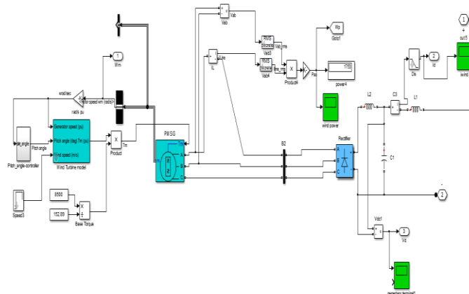
Figure 3: MATLAB Model for Wind System
