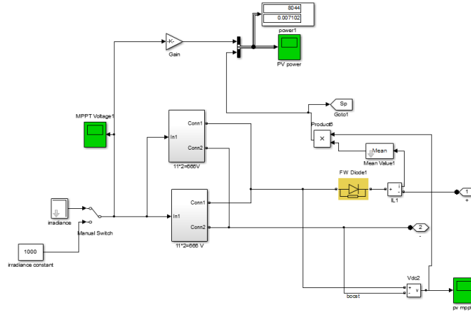
Figure 1: MATLAB Model for PV System
