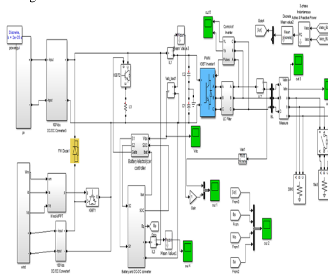
Figure 9: MATLAB Simulink Model of Hybrid Wind-Solar Energy System using MPPT Algorithm
