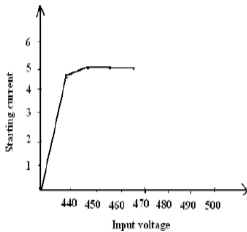
Fig 5. Starting current curve Without Soft Starter
