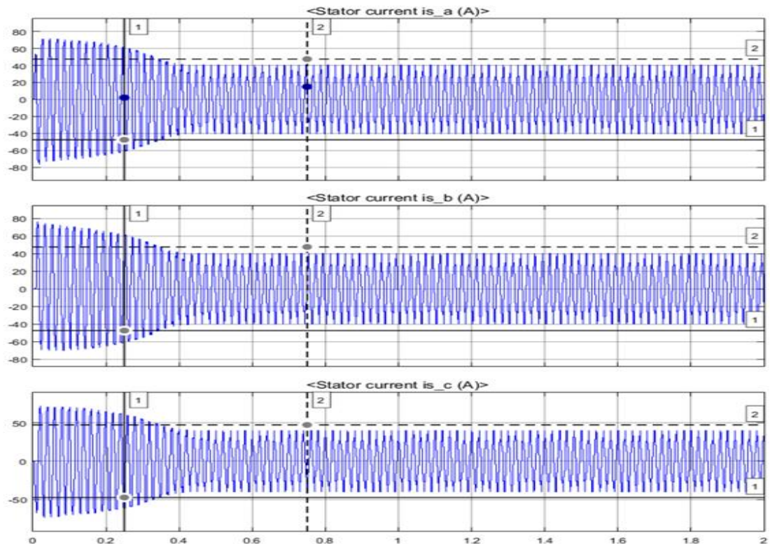
Fig: 8 Stator current versus time characteristics
