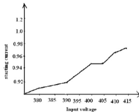
Fig 6. Starting current curve with Soft Starter
