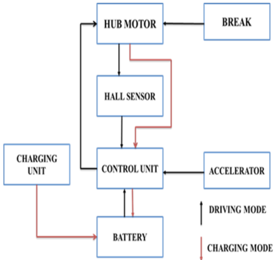
Fig.5. Block Diagram
