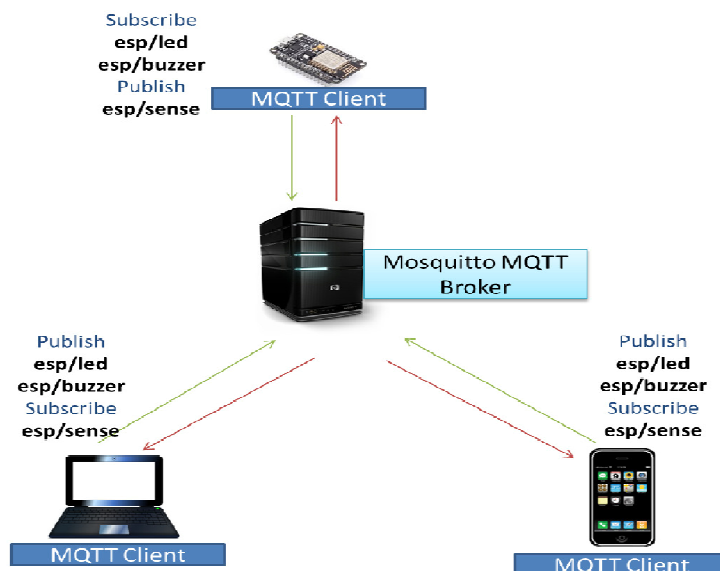
Fig. 4. Message transmission through MQTT
