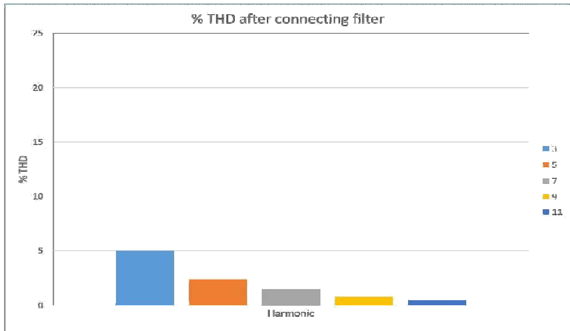
Fig 9: Percentage of THD after connecting filter
