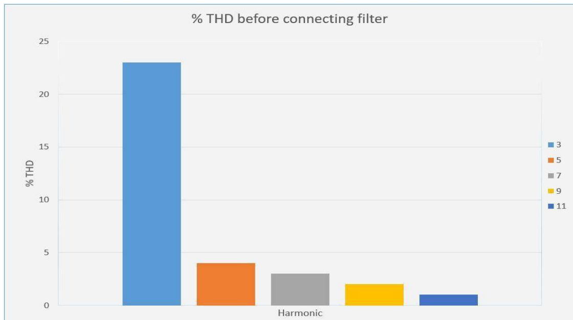
Fig 8: Percentage of THD before connecting filter
