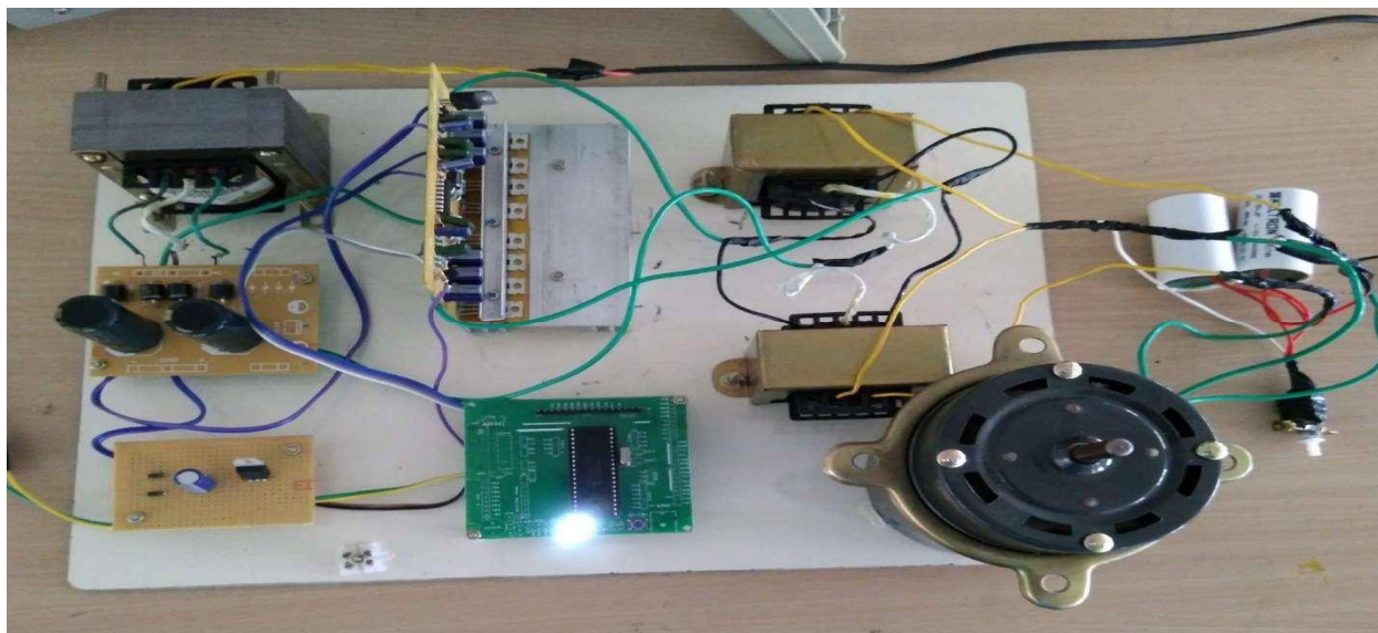
Fig 1: Overall hardware arrangement for reduction of harmonics in three phase transformers
