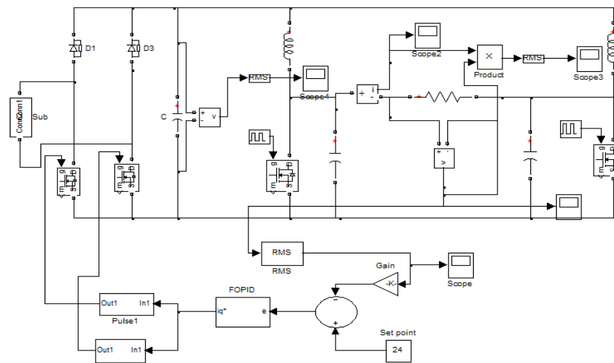
Fig 5 Circuit diagram of the closed loop CEA with FOPID controller
