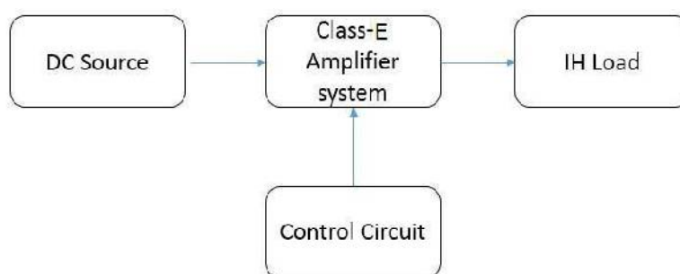
Figure 1.1 Block diagram of the CEA based IH system.
