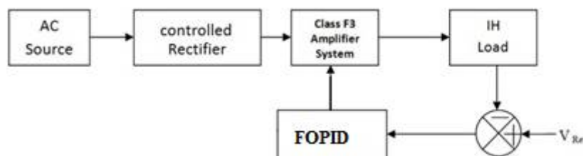
Fig. 2.1 Block diagram of the proposed CEAIHS
