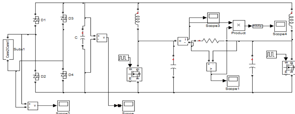
Fig 3 Circuit diagram with disturbance for CEA system
