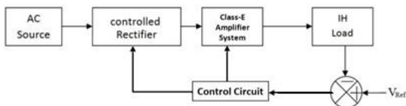
Fig 1.2 Block diagram of the existing IH system
