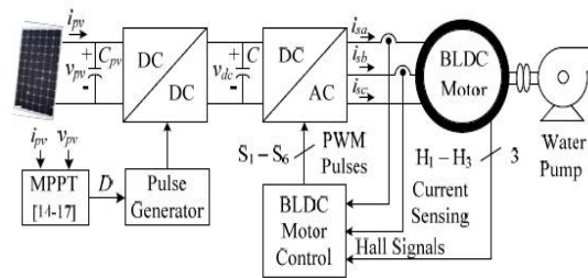
Fig. 1 Conventional SPV fed BLDC motor driven water pumping system.
