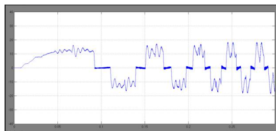
Motor Phase Current Ia
