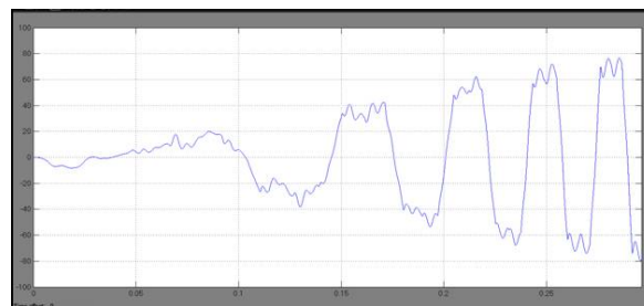
Motor Phase Voltage Ea
