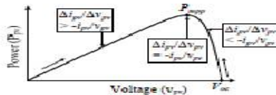
Fig .3 illustration of INC_MPPT with SPV array P_{pv} - V_{pv} characteristics.
