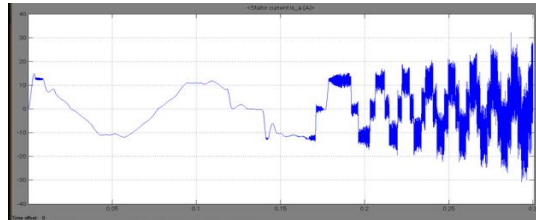
Motor stator current I_a
