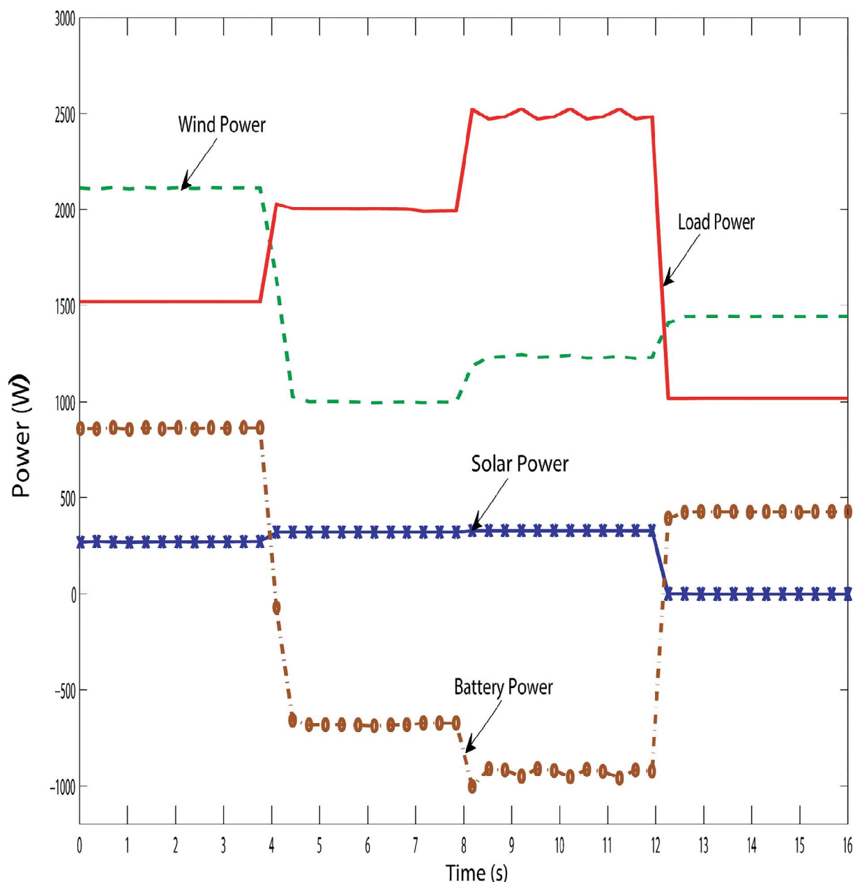
Figure 7: Powers distribution curve of the PV-wind hybrid system during the variation in load with fixed hybrid power.
