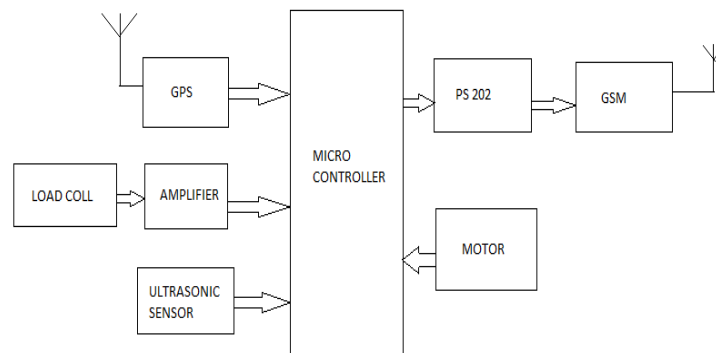
Fig 1.1 Block Diagram of Existing System
