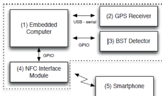
Figure 1. OBU block diagram
