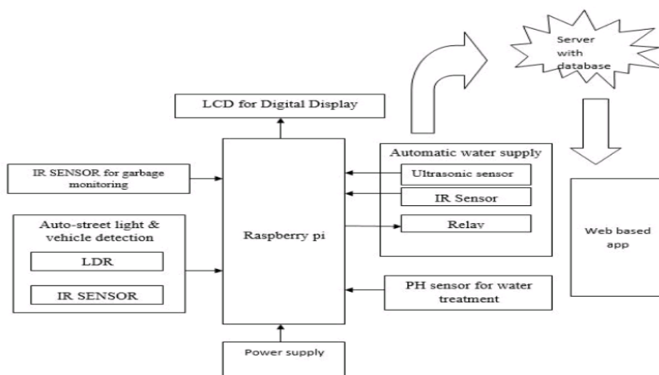
Figure 1 Functional block diagram of the proposed swatch bharat model.
