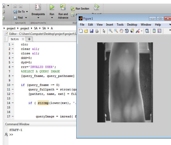
Figure 5. MATLAB output
