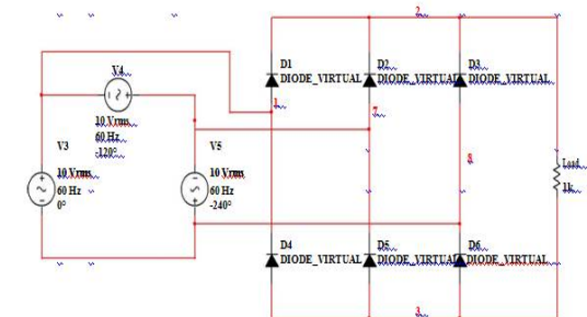
Figure V.9 - Delta Connection
