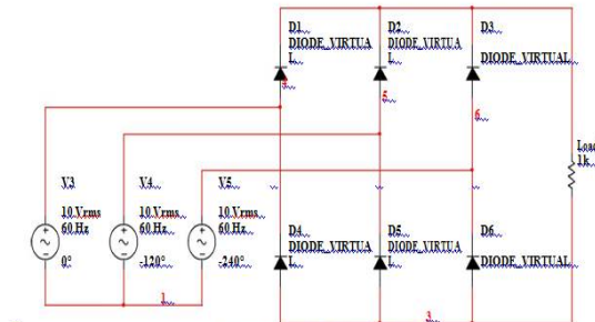
Figure V.8 - Wye Connection
