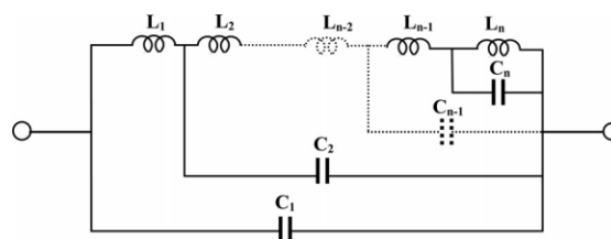
Fig. 3 Double Tuned Resonant Filter
