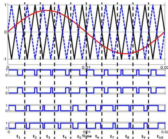
Fig. 8 Modified carrier based PW
