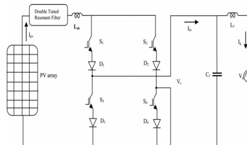
Fig. 1 Single phase grid connected CSI.
