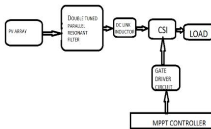
Fig. 2 Block Diagram
