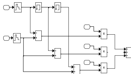
Fig. 8 PID Controller
