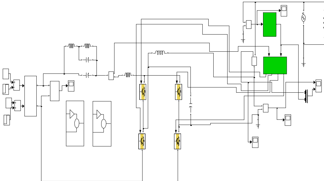
Fig.4 Simulink model for CSI based Grid connected PV system
