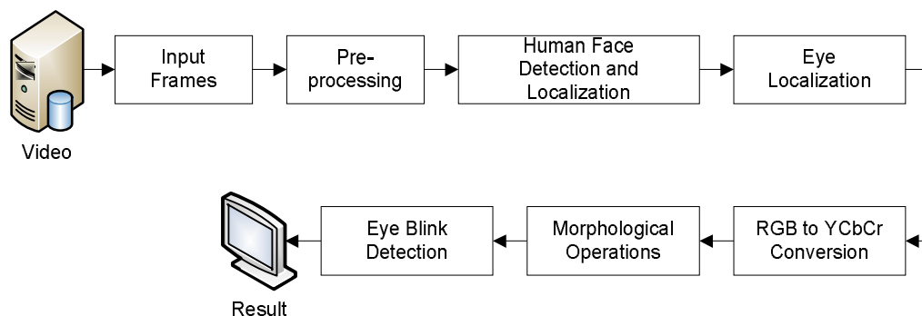
Fig 1: Proposed Architecture
