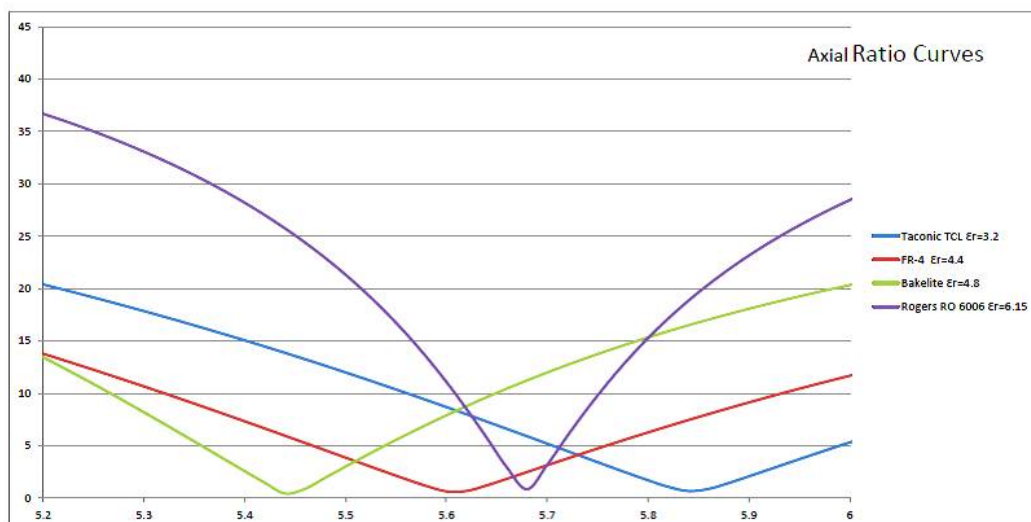
Figure 2: Axial ratio curves for different substrate materials.
