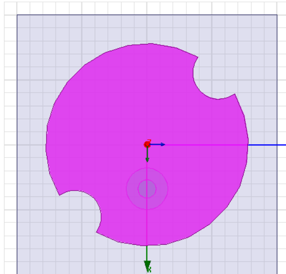
Figure 1: Proposed circular microstrip antenna for circular polarization at 5.9GHz
