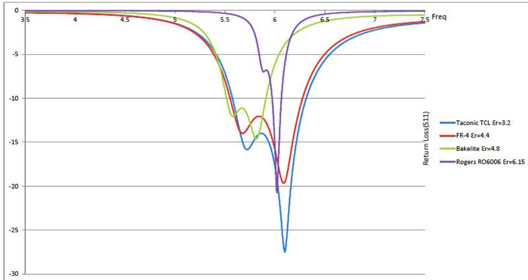
Figure 3: Return loss curves for different substrate materials.
