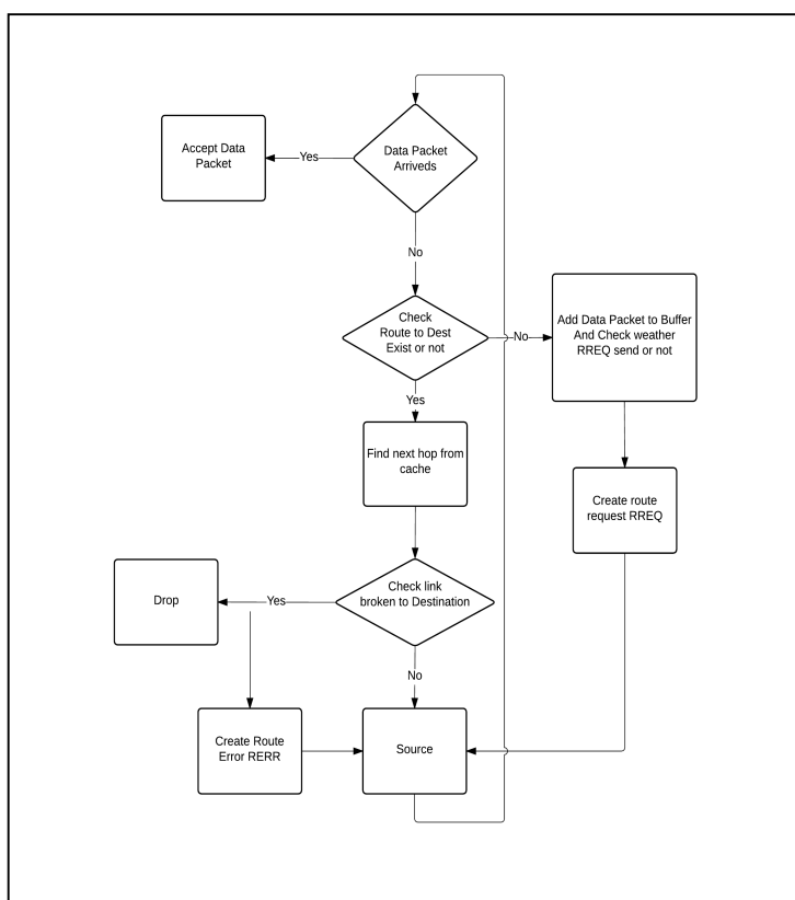
Fig.2. DSR Data flow diagram
