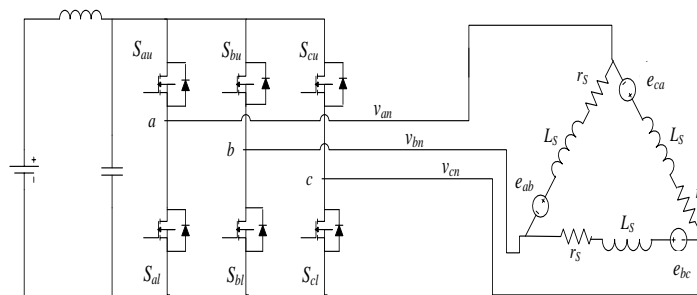
Fig.3 Common voltage-fed inverter topology and motor model
