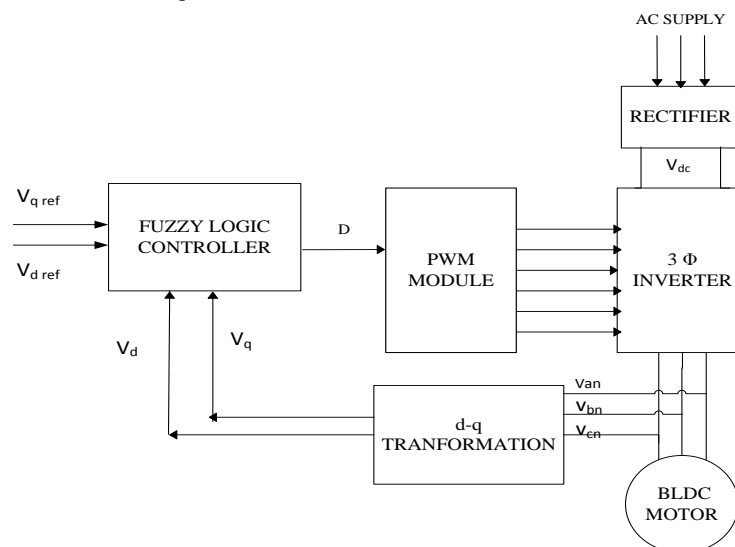
Fig. 1 Block diagram of sensorless Brushless DC motor drives system using Fuzzy Logic controller
