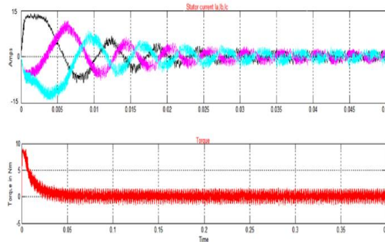
Fig. 5 shows the stator current and developed torque of BLDC motor under fuzzy logic controller
