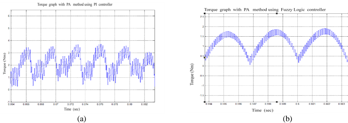
Fig.6 shows (a) Zoomed Torque output of BLDC motor with PA method using PI controller (b) Zoomed Torque output for BLDC motor driven by PA method using fuzzy logic controller
